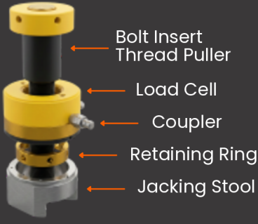
Load Cell Assembly
