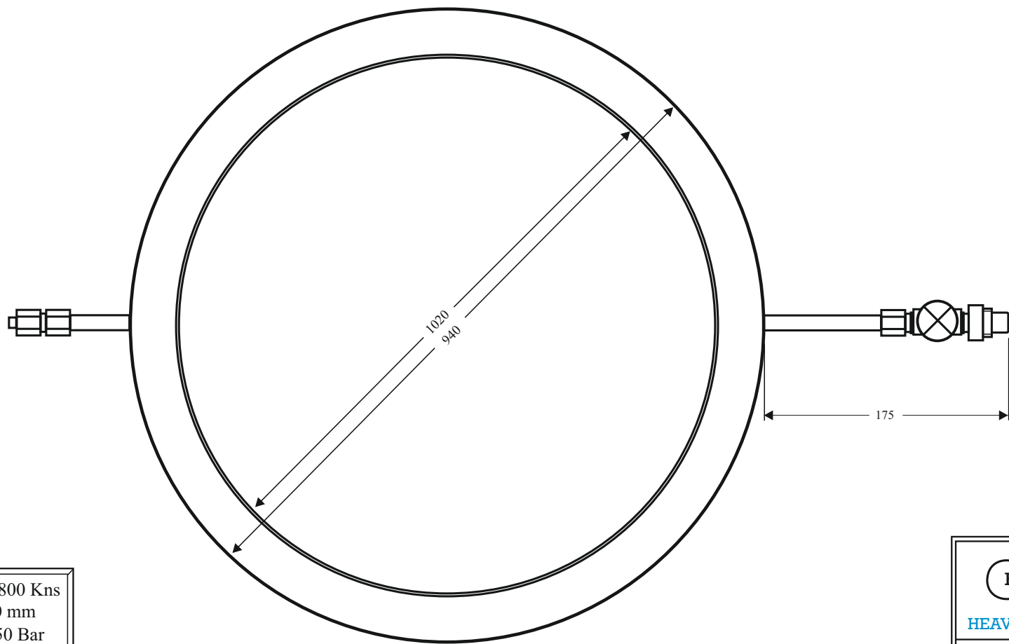
PLAN
