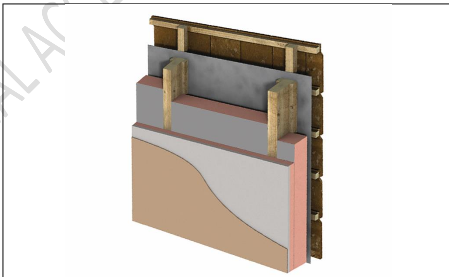
Figure 5 Wetherby internal wall insulation board fixed to metal wall liner
