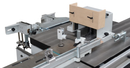
Cuffia a tenonare Revolver Tenoning spindle hood Revolver
