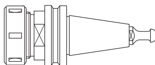
COLLET CHUCKS ISO 30 FOR MULTIAx Page 19
