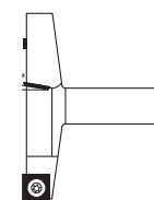
HW INSERT ROUTER BITS FOR PLANING AND RABBETING Page 65
