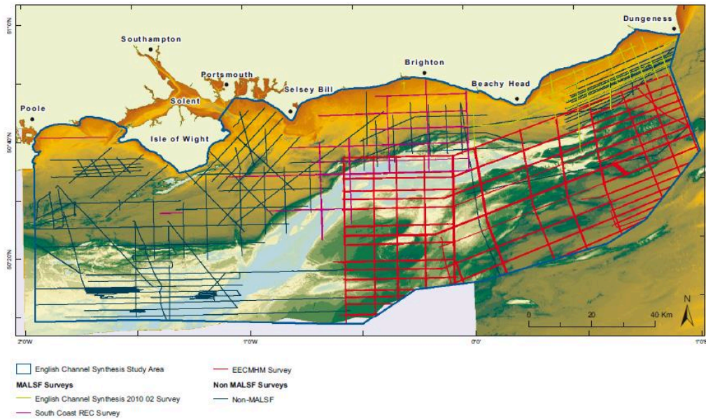
Figure 4 MALSF Synthesis study acoustic remote sensing survey lines (James et al., 2011)
