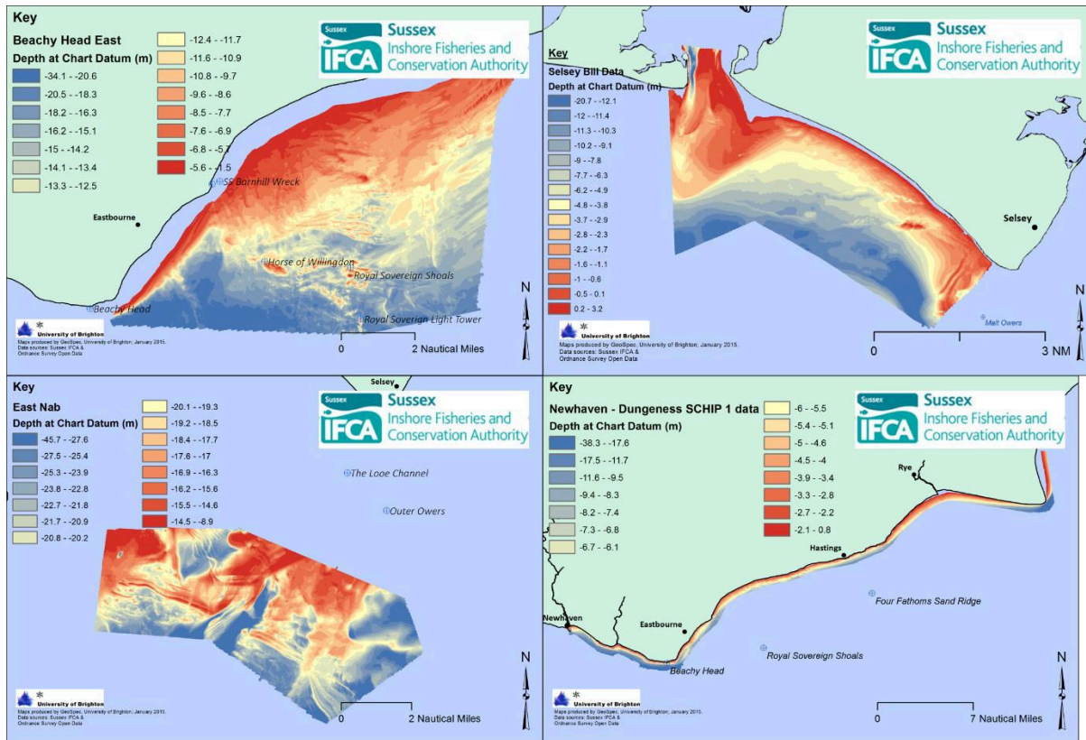
Figure 52 Fine scale bathymetry data. Contains public sector information, licensed under the Open Government Licence v2.0, from the Maritime and Coastguard Agency (National Archives, no date).
