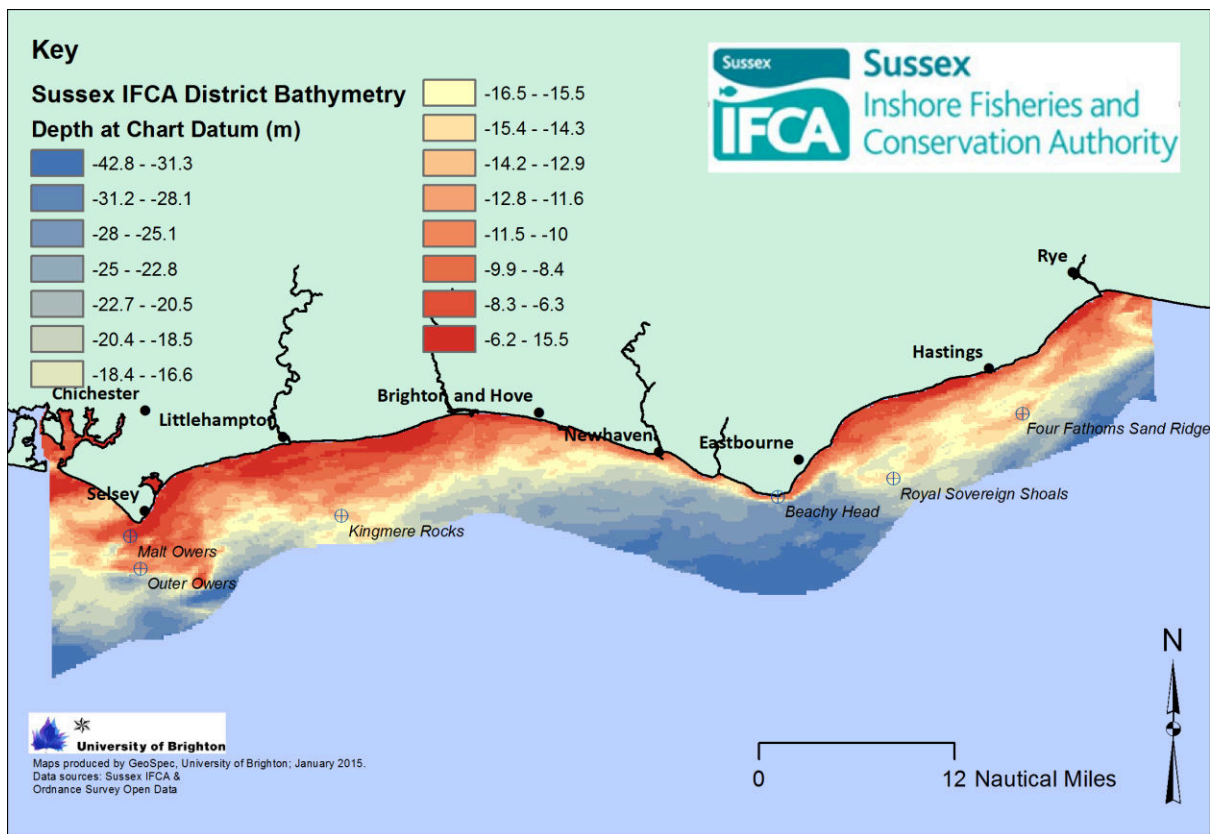
Figure 50 Broad scale bathymetry model for the Sussex IFCA district
