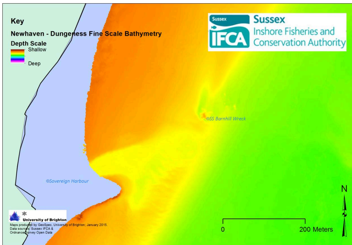
Figure 56 Fine scale bathymetry off of Sovereign Harbour, Eastbourne, showing the SS Barnhill wreck adjacent to the entrance channel. Contains public sector information, licensed under the Open Government Licence v2.0 (National Archives, no date), from CEFAS-
