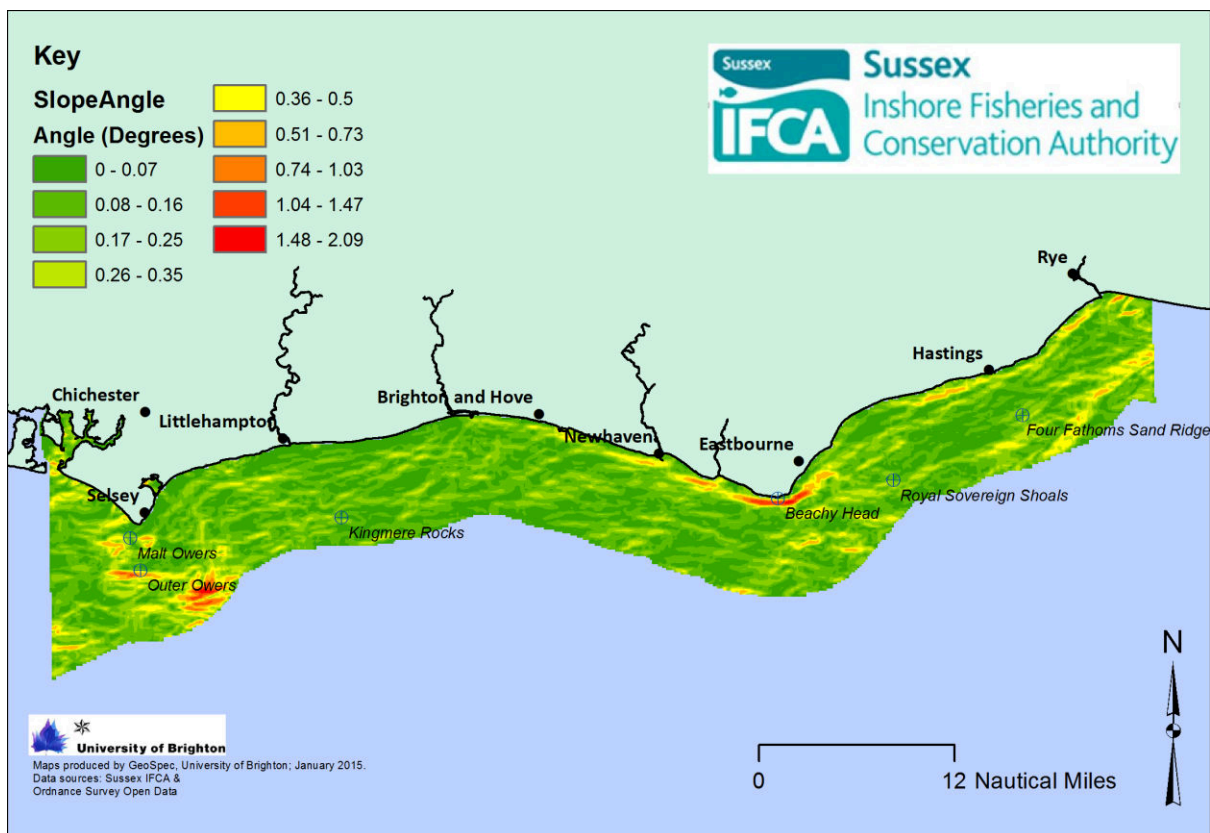
Figure 51 Broad scale slope angle distribution throughout the Sussex IFCA district
