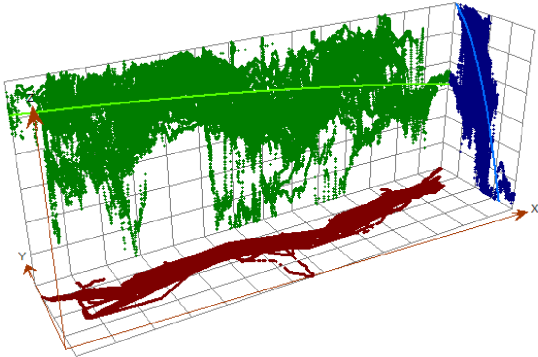
Figure 59 Three dimensional trend analysis for the broad scale bathymetric data, where the Y axis represents longitude, the X axis represents latitude, and the Z axis represents bathymetric depth
