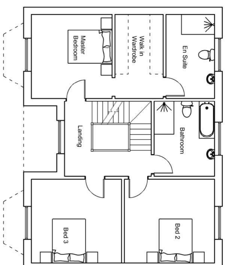
First Floor 1-100
