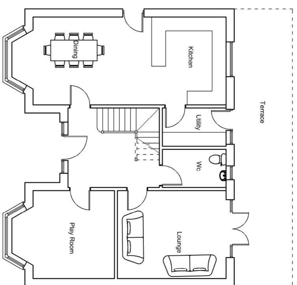
Ground Floor 1-100
