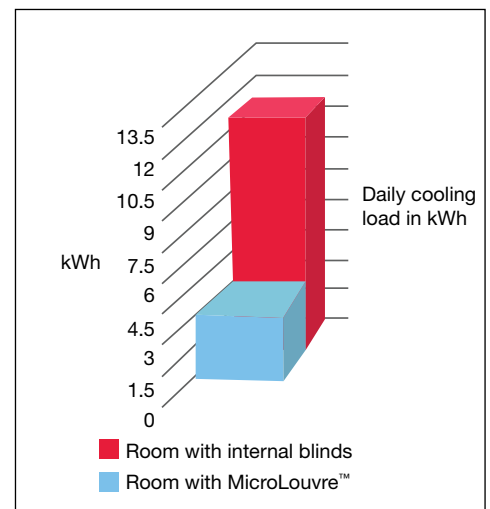
MicroLouvre™ - A fine mesh using woven bronze louvres provide 100% solar protection with a sun angle of 40° or more, with 80% free area and maximum vision to the external environment.
