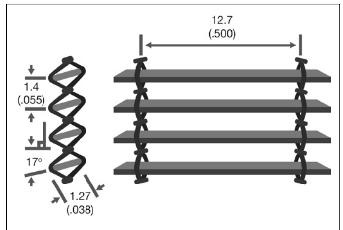
MicroLouvre™ - A fine mesh using woven bronze louvres provide 100% solar protection with a sun angle of 40° or more, with 80% free area and maximum vision to the external environment.
